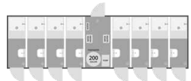
FLOOR PLAN
